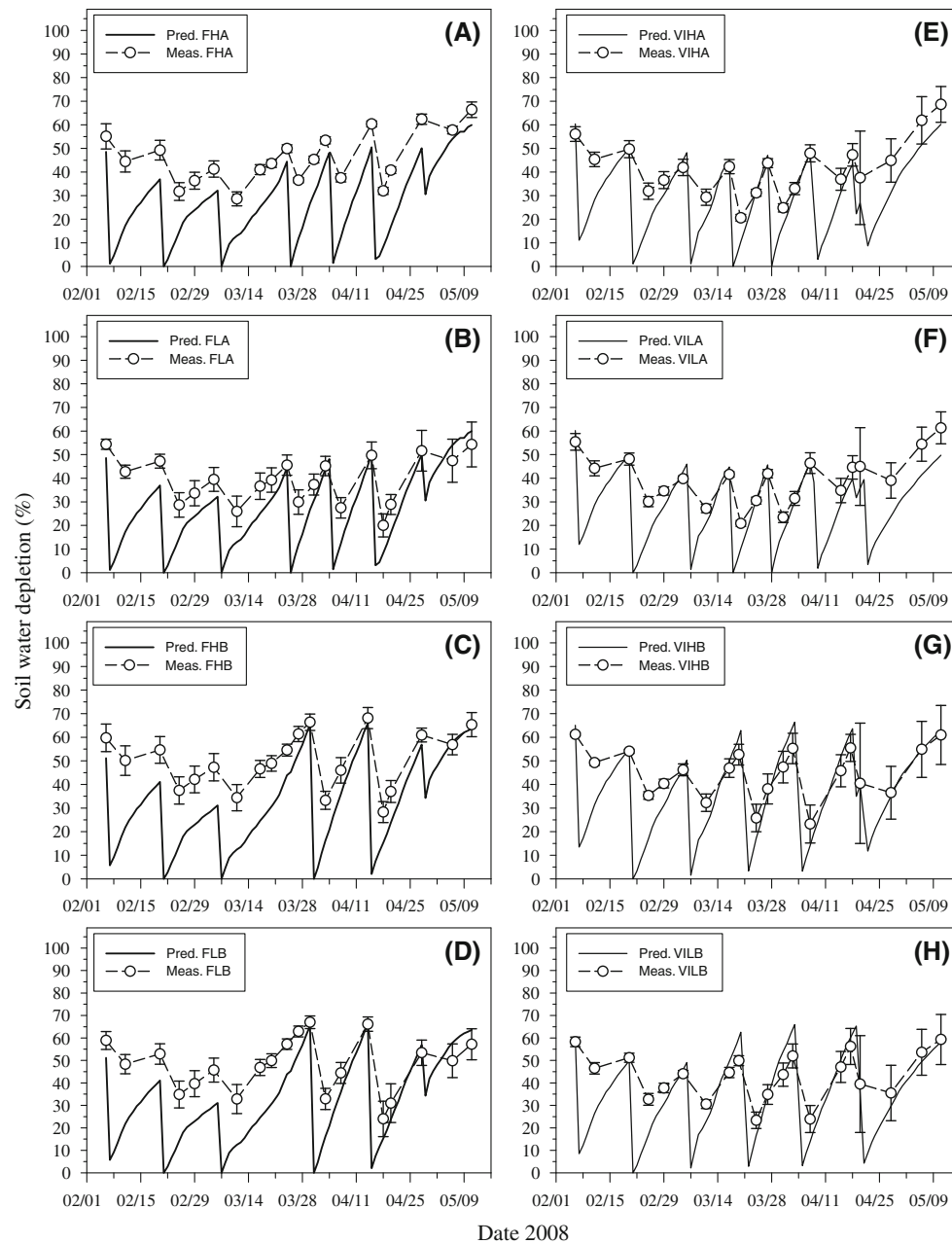
Fig. 5 Mean predicted and mean measured soil water depletion with time for sub-treatment FHA (a), FLA (b), FHB (c), FLB (d), VIHA (e), VILA (f), VIHB (g), and VILB (h) in the 2008 experiment. Error bars about the measured means indicate the standard deviation
