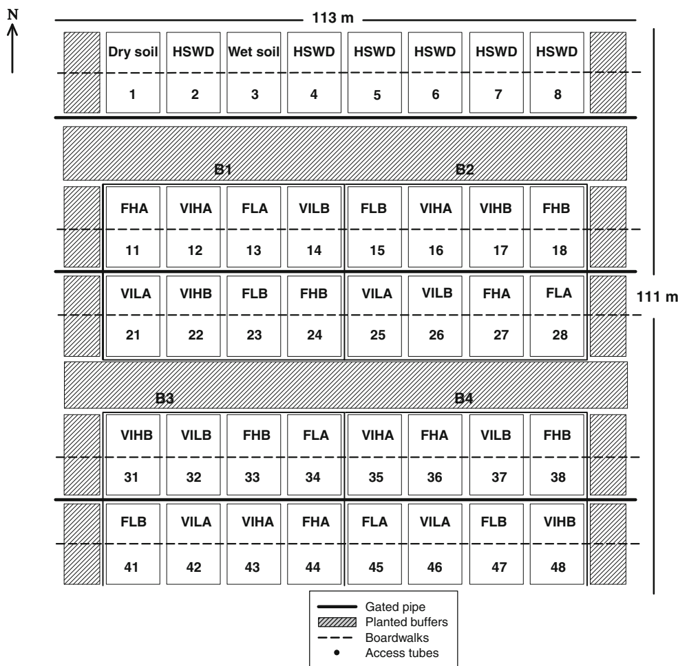
Fig. 1 Camelina experiment field site at Maricopa, Arizona, showing 40 plots, each 10 m × 17 m. Acronyms (defined in Table 1) shown at the top of each plot correspond to the particular sub-treatment for the plot within the 2 × 2 × 2 factorial. The eight sub-treatments were
